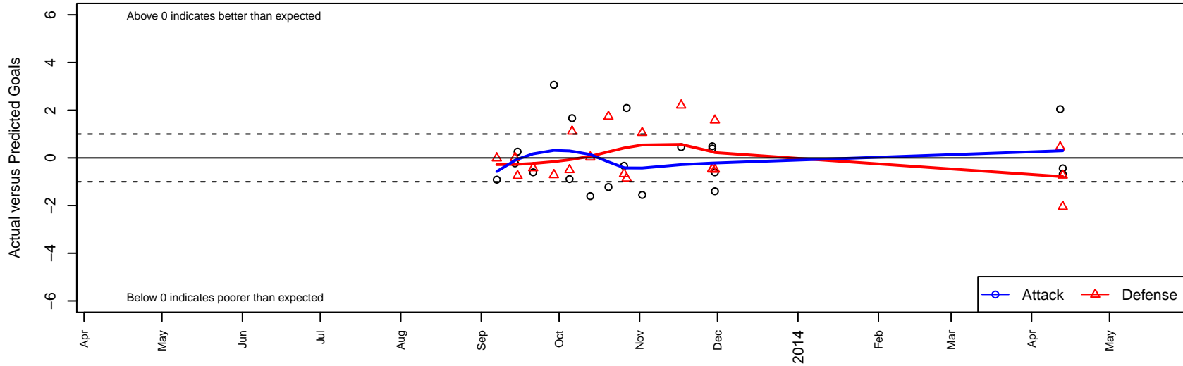
PCSC Red B97 Dots are actual minus expected GF (blue circles) and GA (red triangles). Blue line is smoothed change in attack strength. Red is smoothed change in defense strength.
